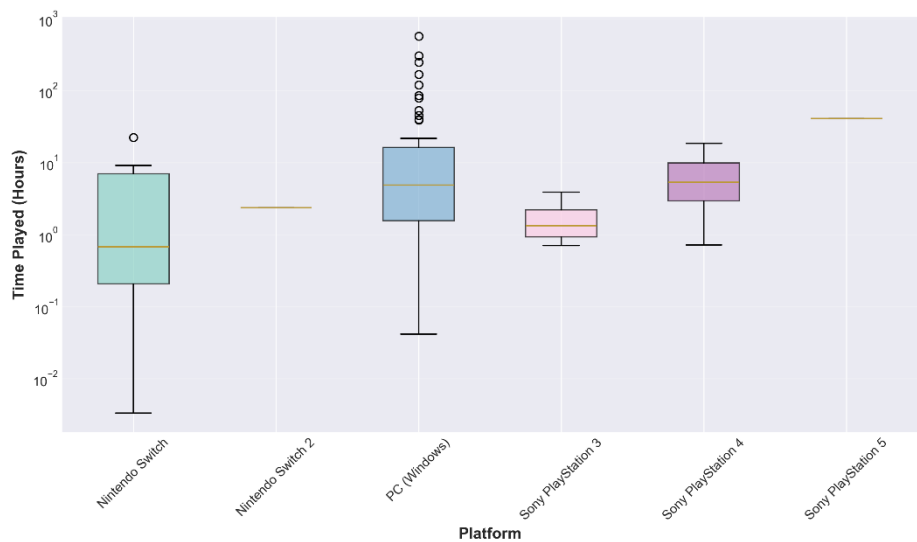
Fig. 7. Platform Distribution
